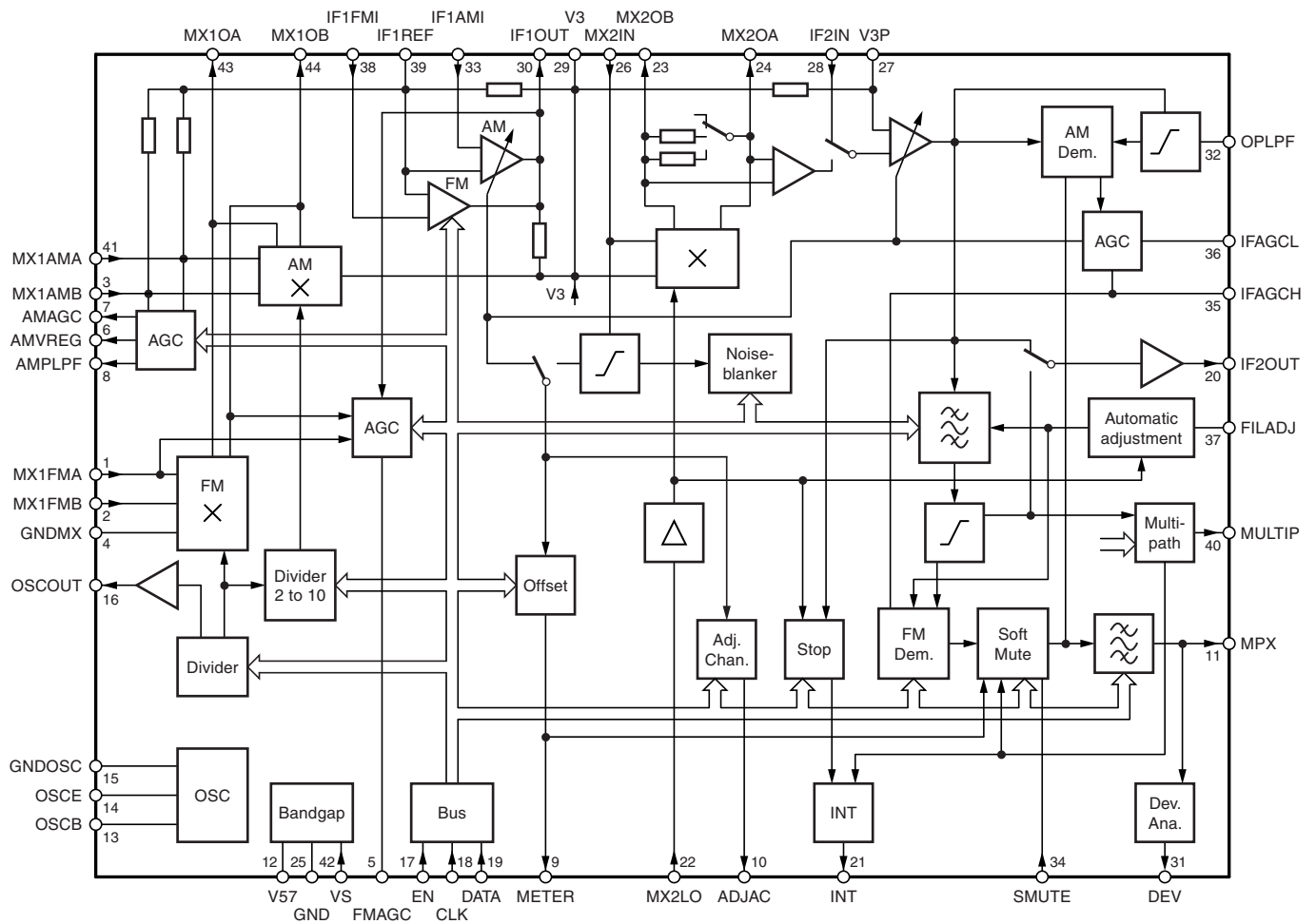
Figure 1-1. Block Diagram
