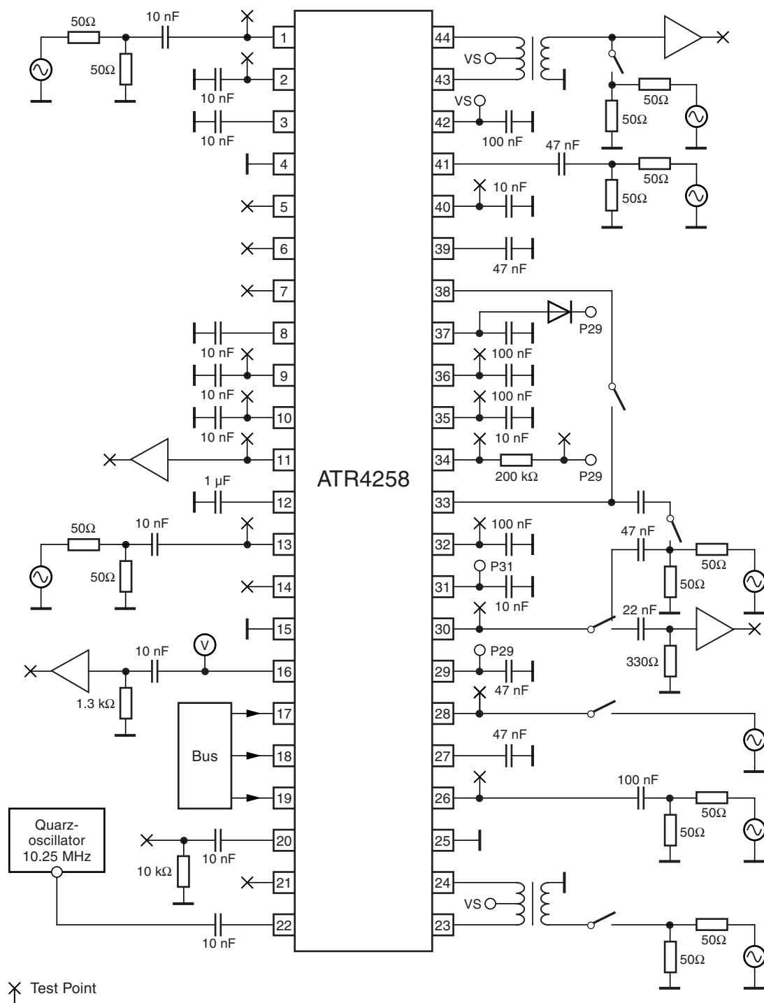
Figure 10-8. Test Circuit
